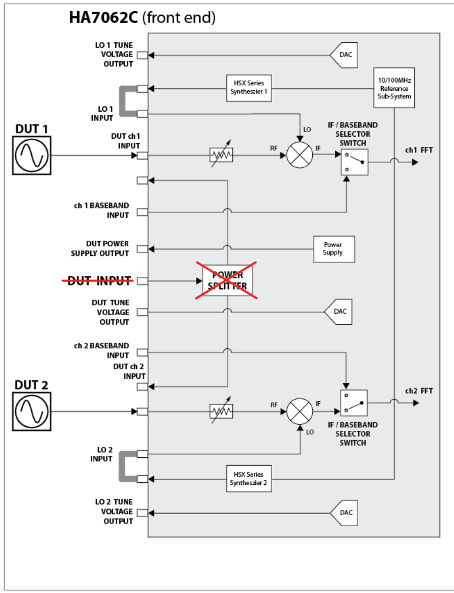
Figure 2: HA7062C Noise Floor Measurement Block Diagram
