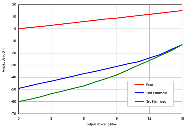
Figure 6: Absolute Harmonic Data ( F_0 = 1\text{GHz} )
