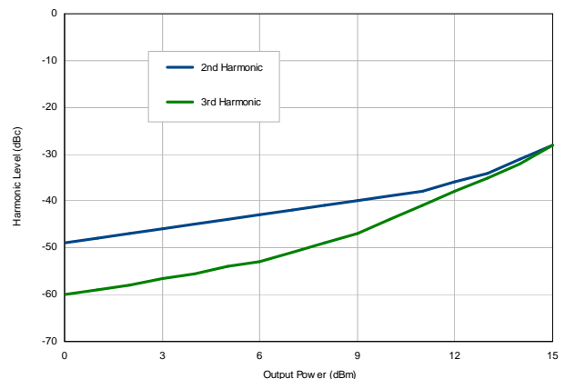
Figure 7: Relative Harmonic Data ( F_0 = 1\text{GHz} )
