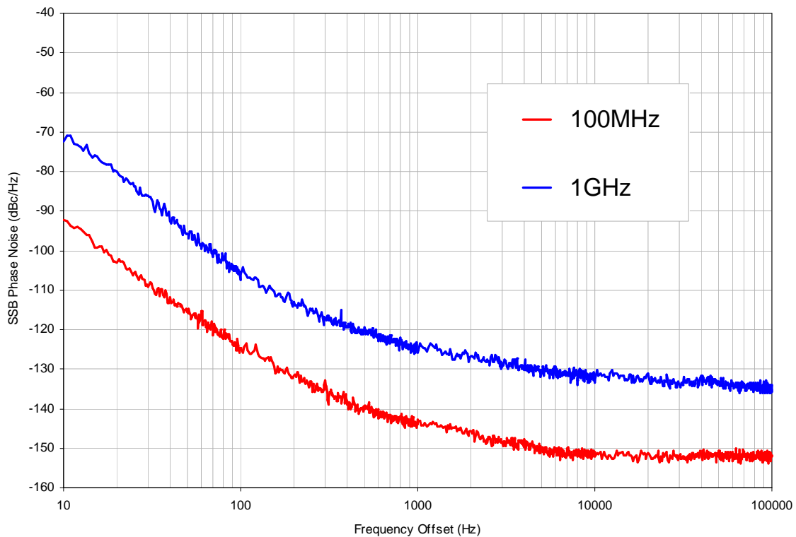
Figure 1: SSB Phase Noise at 100MHz & 1GHz ( P_{OUT}=+12dBm )
