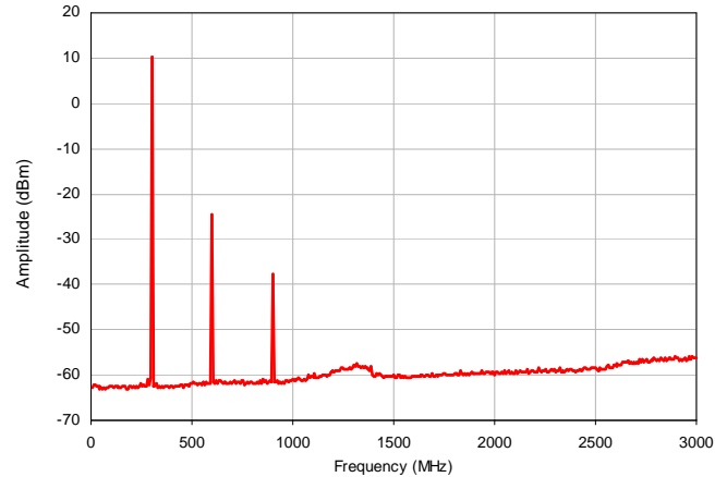
Figure 4: Spectral Data at 300MHz ( P_{OUT} = +10\text{dBm} )
