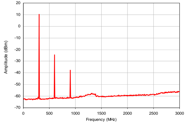
Figure 6: Spectral Data at 300MHz ( P_{OUT} = +10\text{dBm} )
