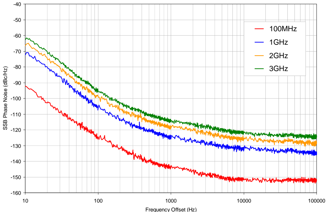
Figure 1: SSB Phase Noise at 100MHz, 1GHz, 2GHz & 3GHz ( P_{OUT}=+12dBm )
