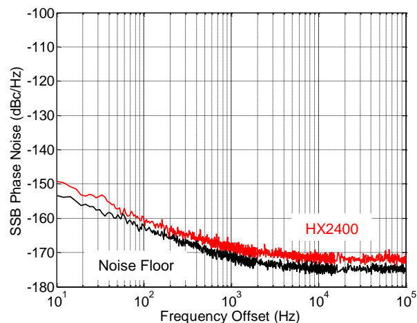
Figure 4: SSB Phase Noise at 100MHz ( P_{IN} = +4 dBm)
